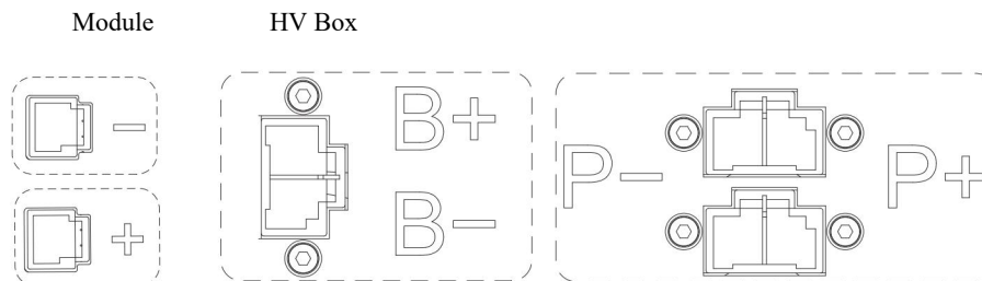
Figure 5-2 Power ports
